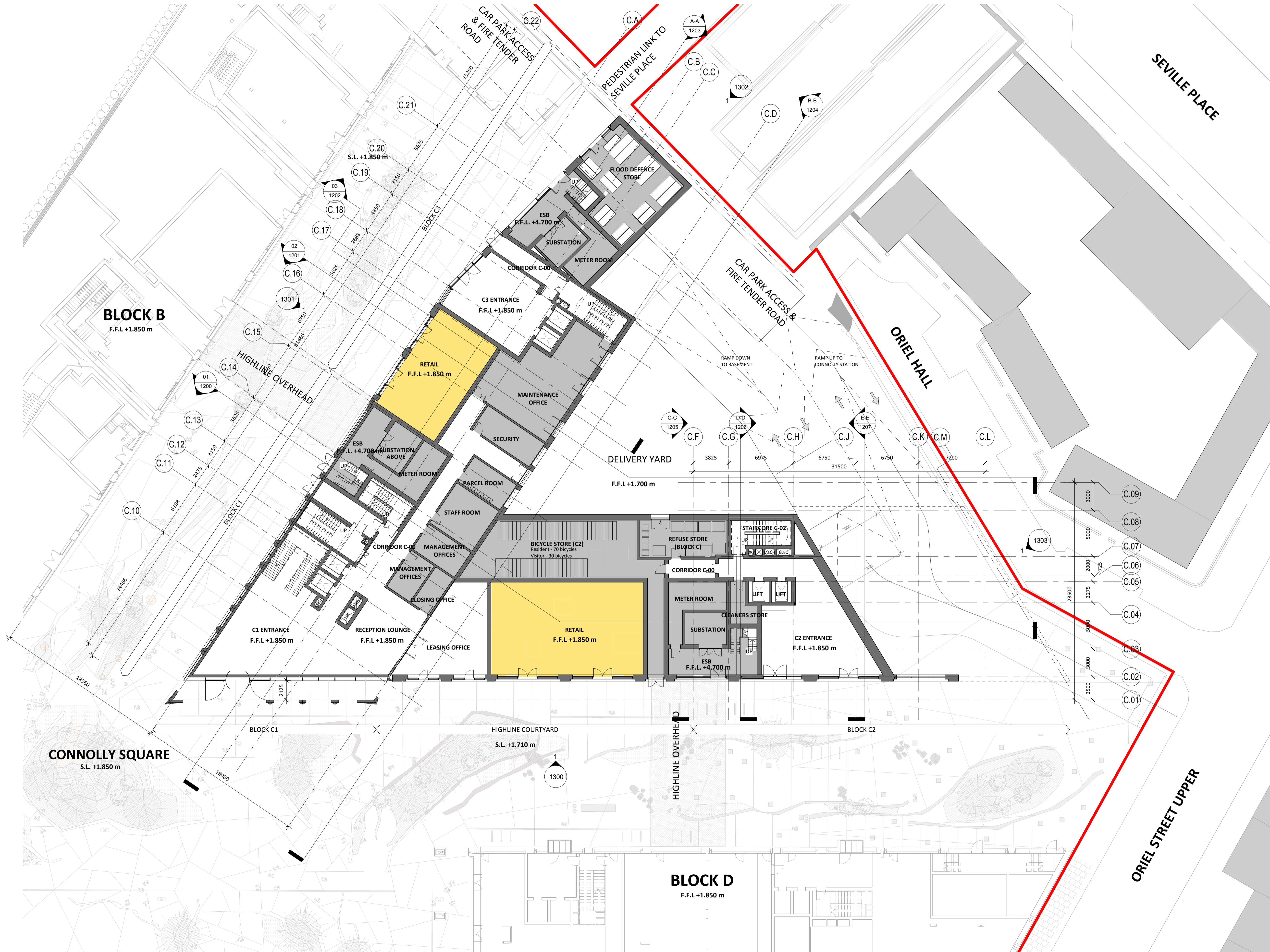
1 BLOCK C PLAN_LEVEL 00 1 : 200
